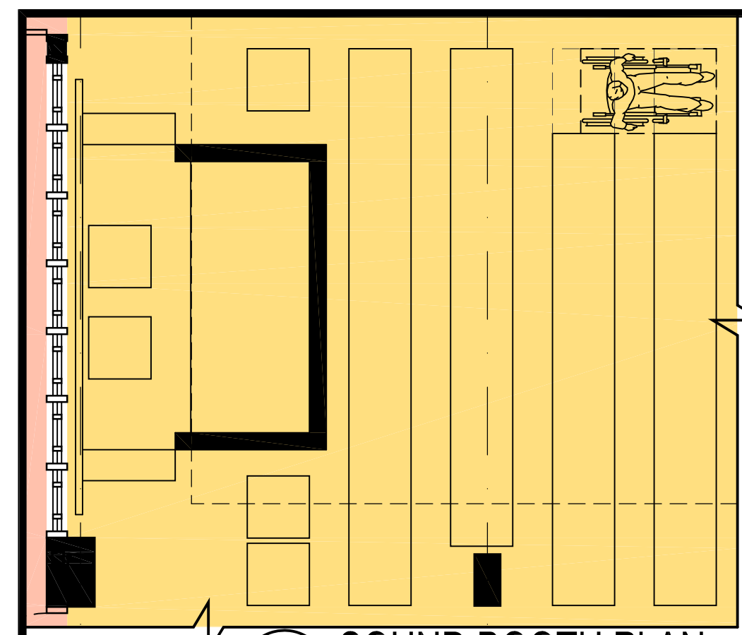
D SOUND BOOTH PLAN A1.4 SCALE: 1/4" = 1'-0"
