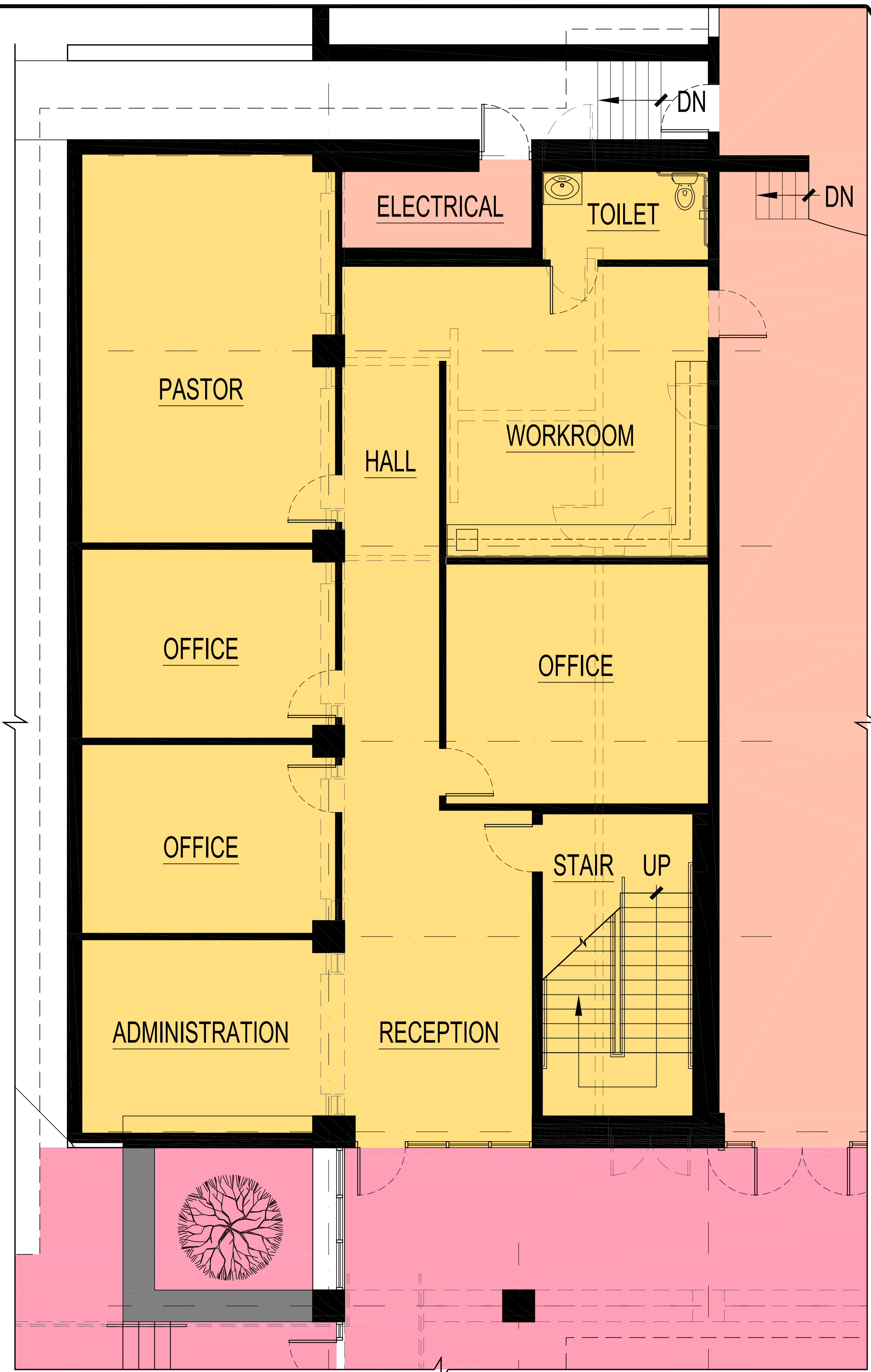
B ADMINISTRATION PLAN A1.4 SCALE: 1/4" = 1'-0"
